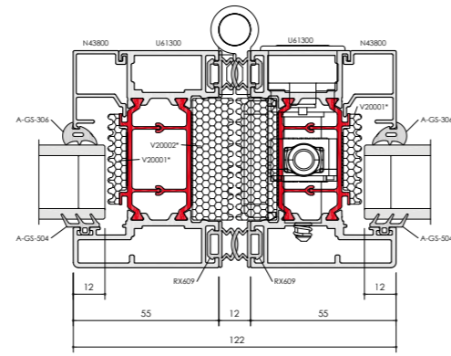
F82 MEETING STYLE / B
