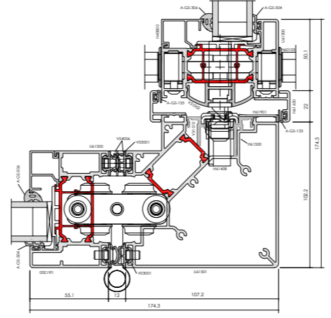
F82 FLOATING CORNER POST / C1
