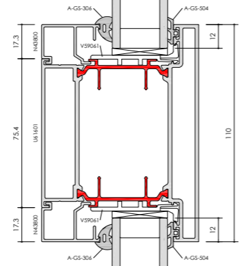
F82 MIDRAIL / E
