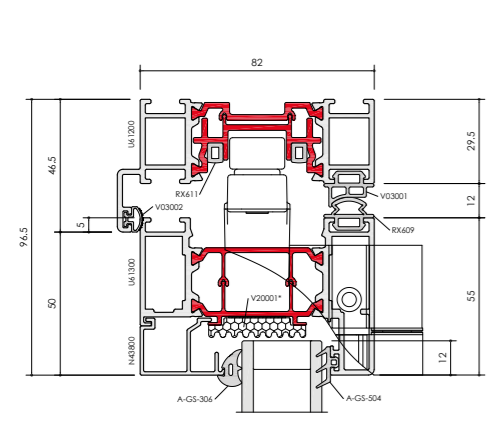
F82 HEAD / A
